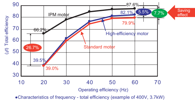
• Characteristics of frequency - total efficiency (example of 400V, 3.7kW)
